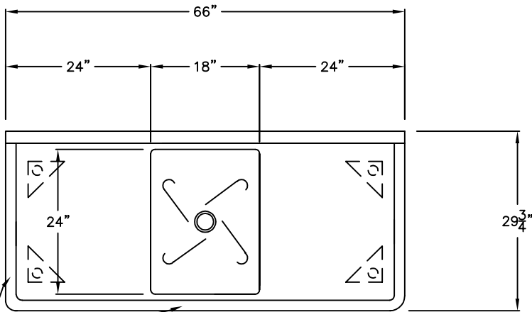
1 3/4" ROLLED EDGE FRONT & ENDS PLAN VIEW
