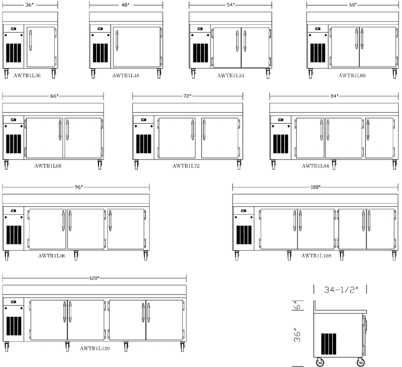
STANDARD PROFILE
