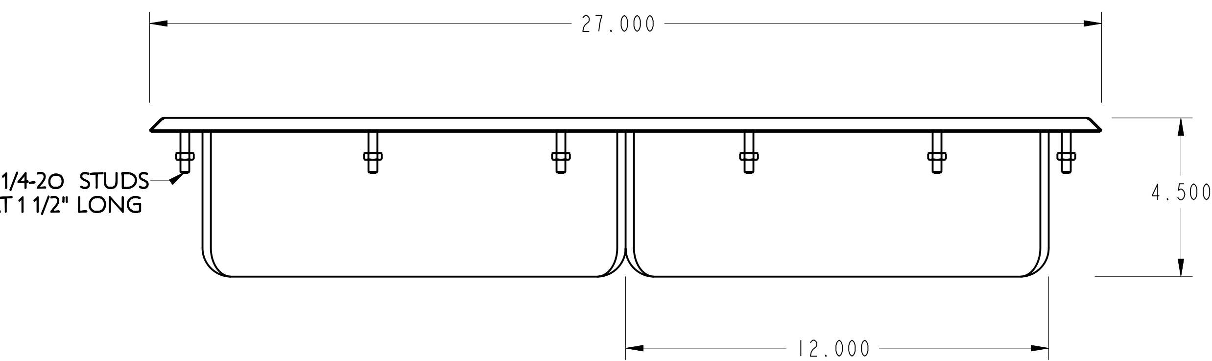
FRONT ELEVATION
