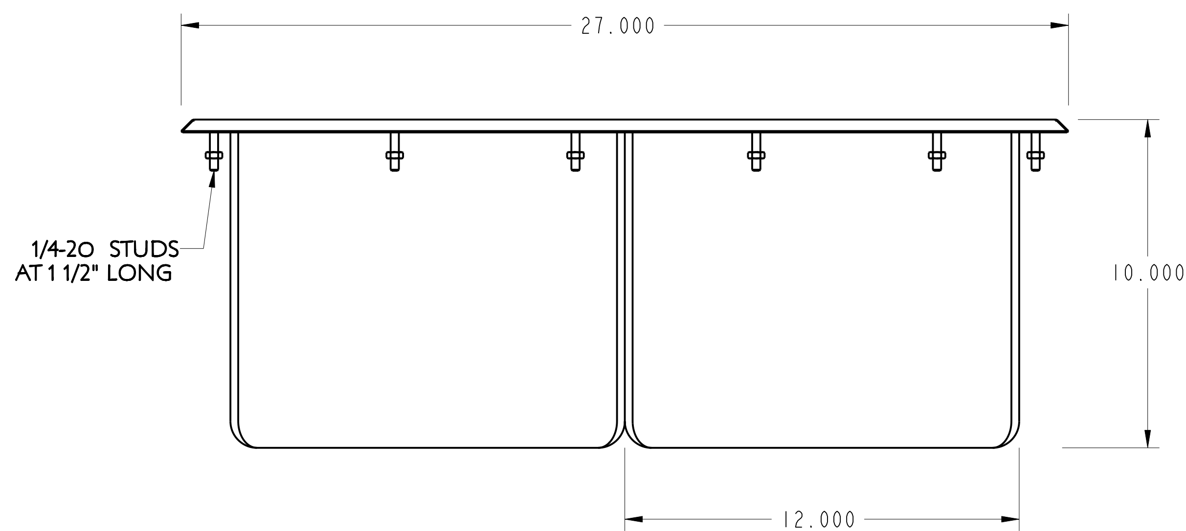
FRONT ELEVATION
