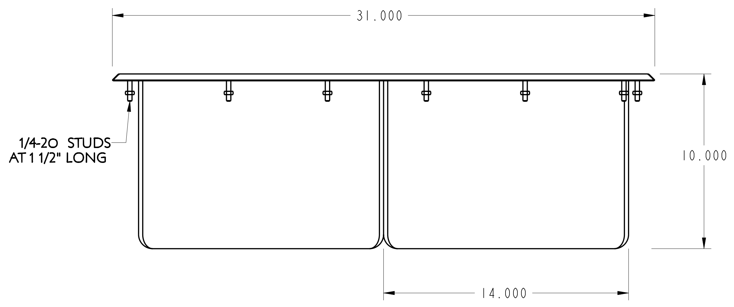
FRONT ELEVATION
