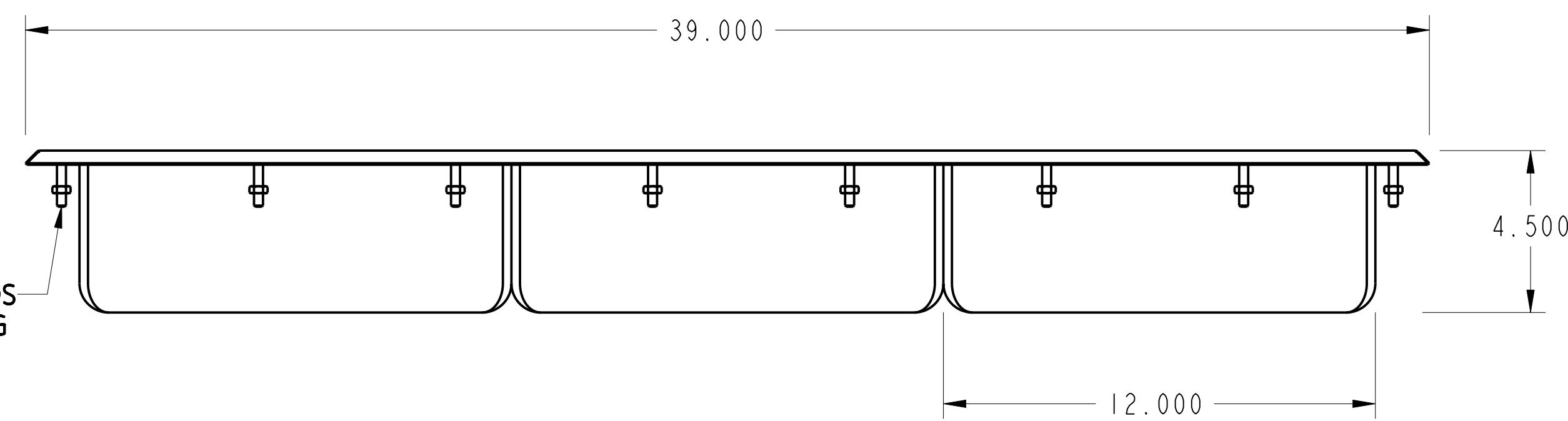
FRONT ELEVATION
