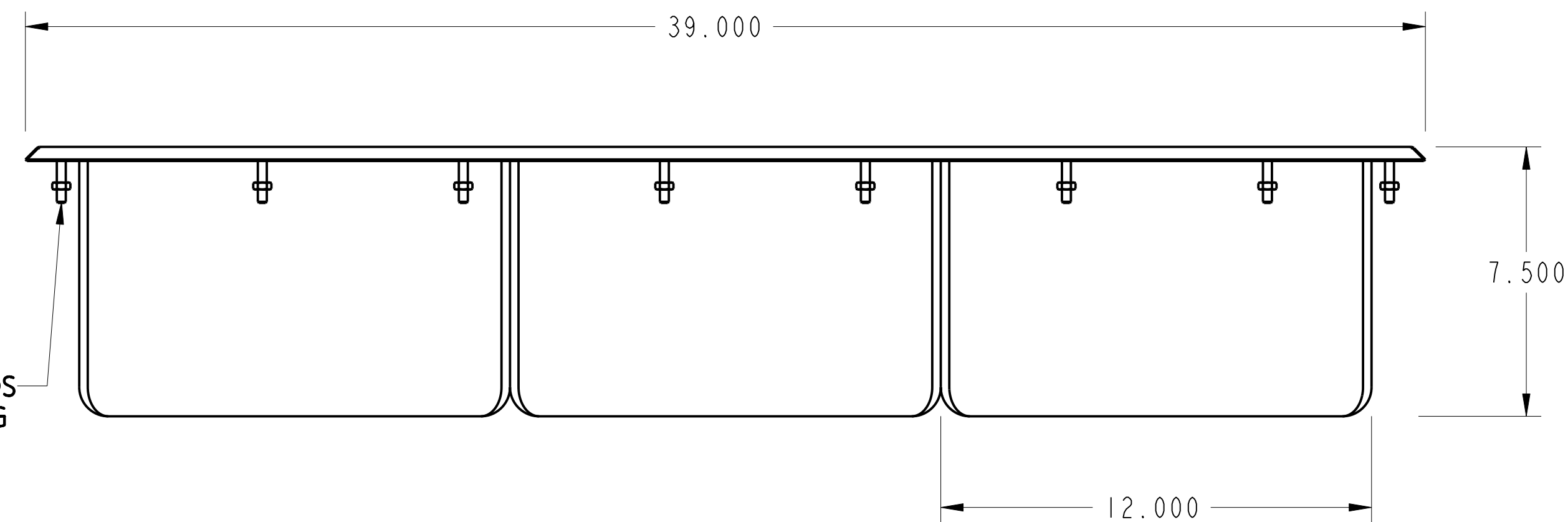
FRONT ELEVATION
