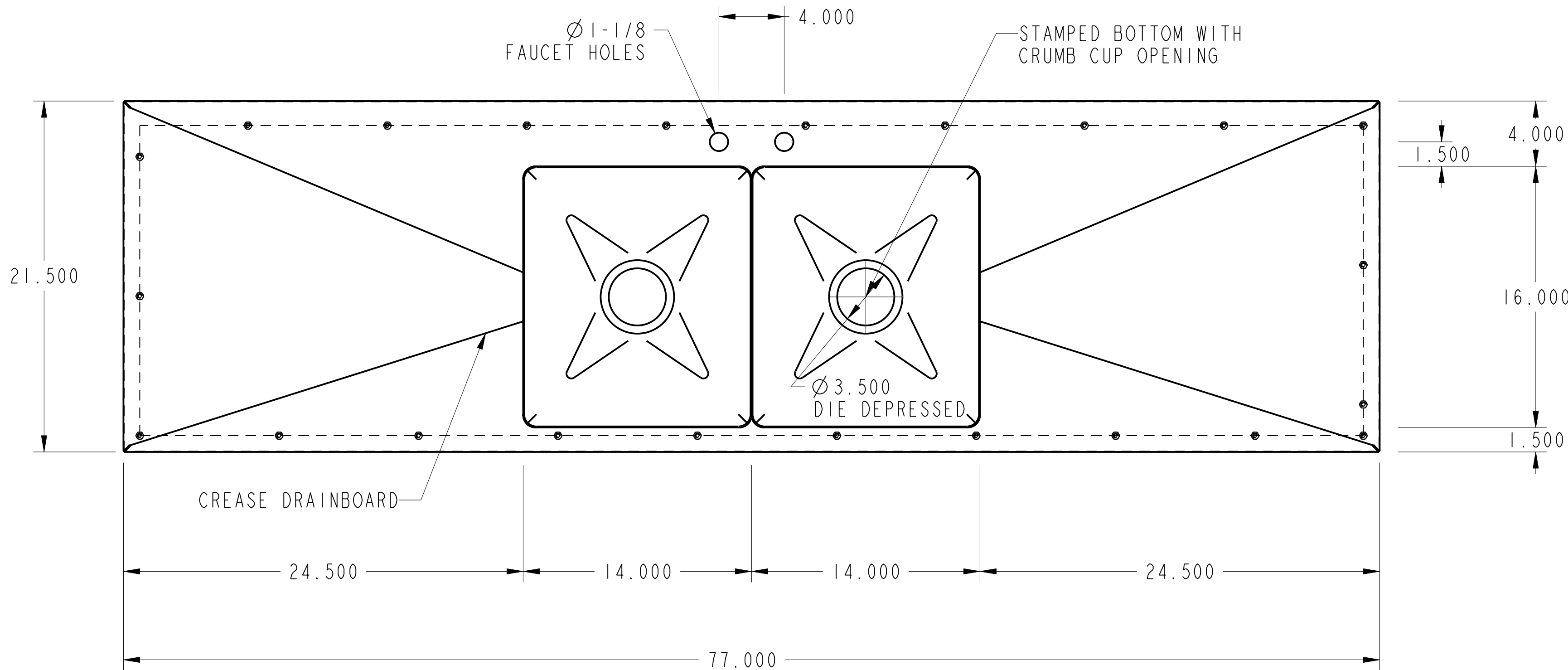
PLAN VIEW
