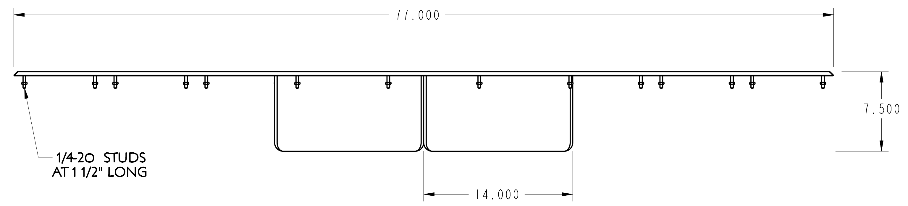
FRONT ELEVATION
