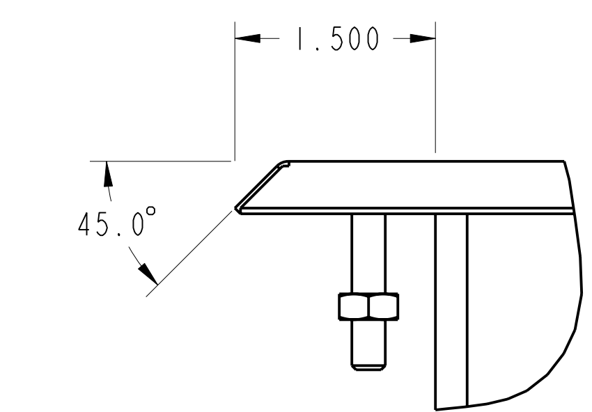
DETAIL A SCALE 1.000
