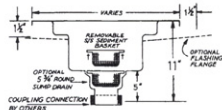
TROUGH INSTALLATION WITH OPTIONAL FLASHING FLANGE & SUMP DRAIN
