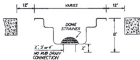
CONCRETE BLOCKOUT FOR FUTURE INSTALLATION
