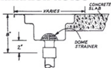
INSTALLATION AT TIME OF CONCRETE POUR
