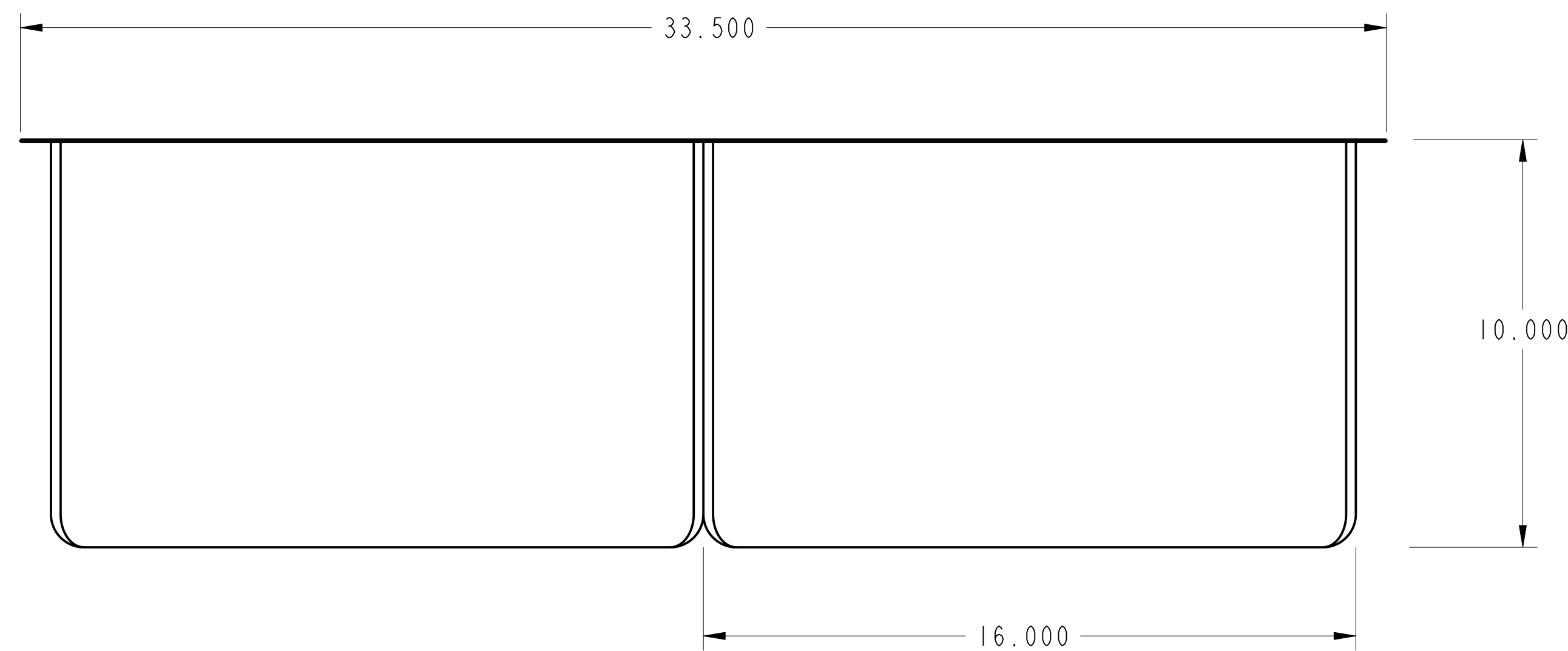
FRONT ELEVATION
