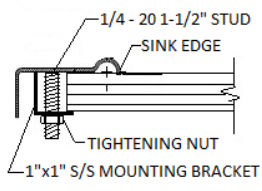
DETAIL SECTION
