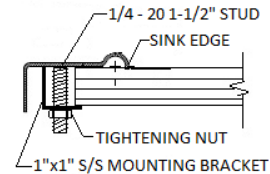
DETAIL SECTION
