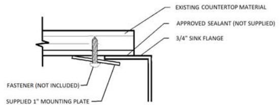
DETAIL SECTION
